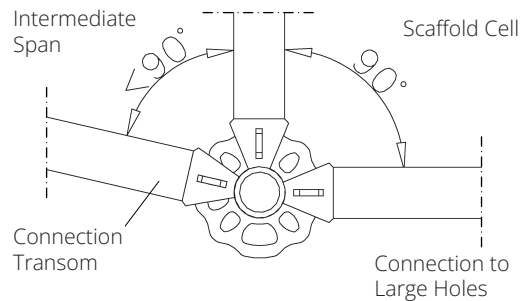
Junction Detail
