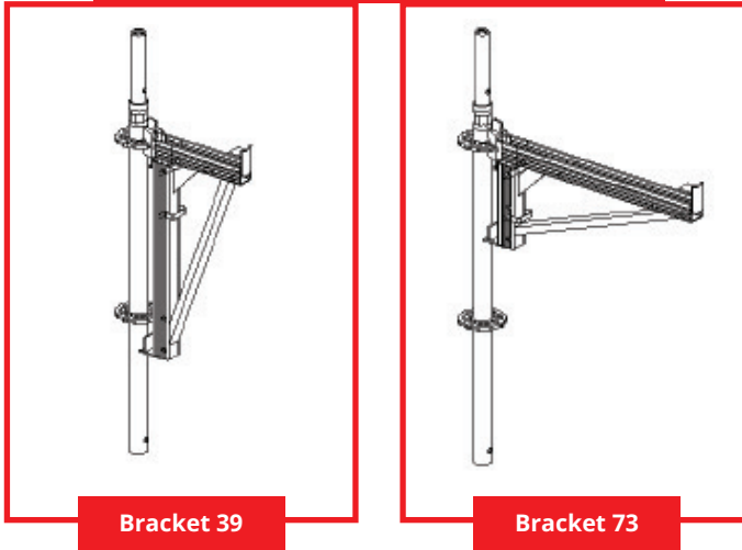
Figure 41: Adjustable Bracket 39/73 (U Support)
